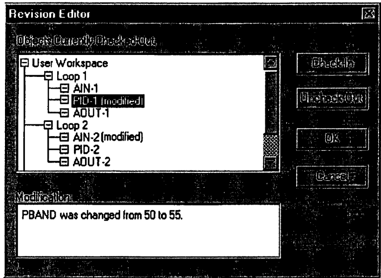
Figure 48 - Revision Editor
